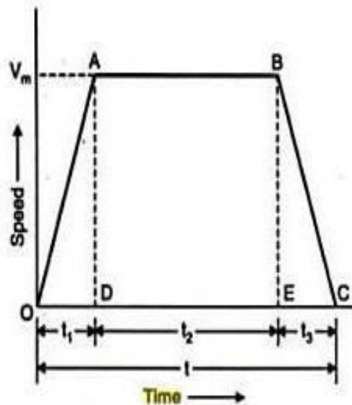
Trapezoidal speed-time curve.
